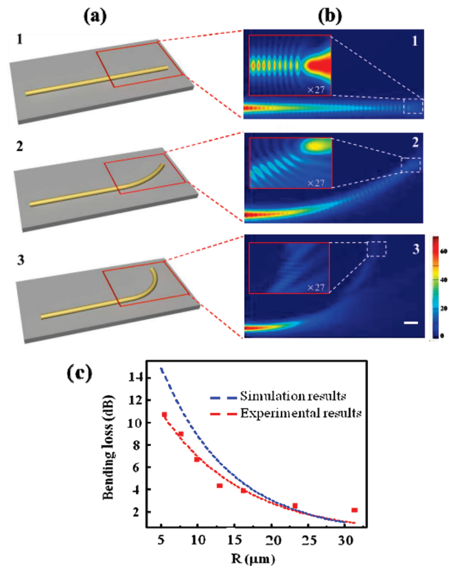
Figure 3. The calculated distribution of electric field intensity around a Ag NW by the FDTD method. (a) Schematics of a Ag NW when it is straight in (a) 1, and bent with bending radius of 25 \mu\text{m} in (a) 2 and 10 \mu\text{m} in (a) 3. (b) The calculated electric field distribution. The insets show the corresponding distribution of electric field intensity at the output end of Ag NW. The maximum intensity of color bar in the inset is 27 times lower than that of the color bar shown on the bottom. The scale bar is 1 \mu\text{m} . (c) The calculated bending loss as a function of bending radius (in blue). The observed experimental results as in Figure 2c are also shown for comparison (in red).
