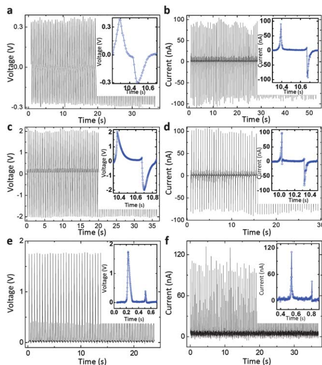
Fig. 2 Electrical characteristics of fabricated nanogenerators as they are periodically strained and released. (a) Open-circuit voltage output of a fabricated nanogenerator. (b) Closed-circuit current output of a fabricated nanogenerator. (c) Open-circuit voltage output of ten-layer integrated nanogenerators. (d) Closed-circuit current output of ten-layer integrated nanogenerators. (e) Rectified open-circuit voltage output of ten-layer integrated nanogenerators. (f) Rectified closed-circuit current output of ten-layer integrated nanogenerators.
