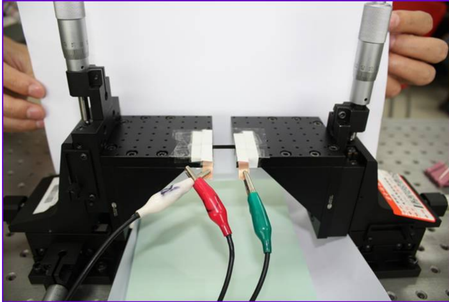
Figure S1. Setup for the conductance measurement of carbon fabric with different curvature.
