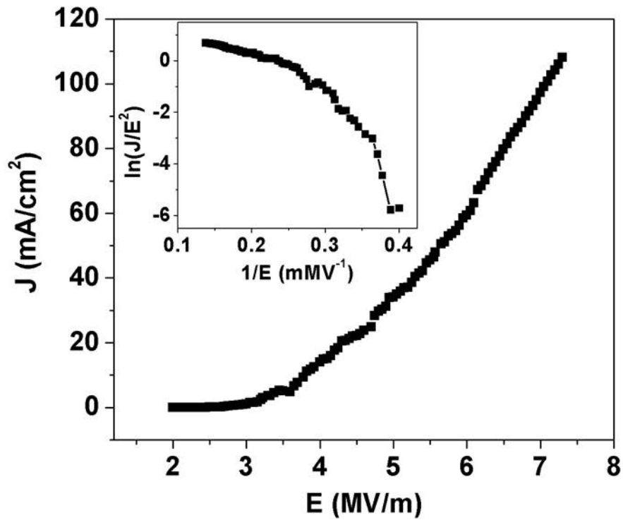
Figure S2. Field emission current density versus electric field of CNPs on carbon fabric. The left inset is the corresponding F-N curves.
