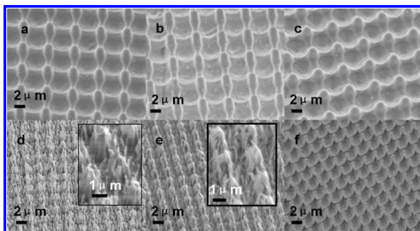
Figure 6. Effect on patterns and PNWs arrays of Dura film with different laser powers: (a, b, c) 2.5 \mu\text{m} period of patterns on Dura film with laser power of 40, 90, and 110 \text{mJ}/\text{cm}^2 , respectively; (d, e, f) 2.5 \mu\text{m} period of PNWs on Dura film with laser power of 40, 90, and 110 \text{mJ}/\text{cm}^2 , respectively. Insets are the enlarged view of PNWs in each picture, respectively.
