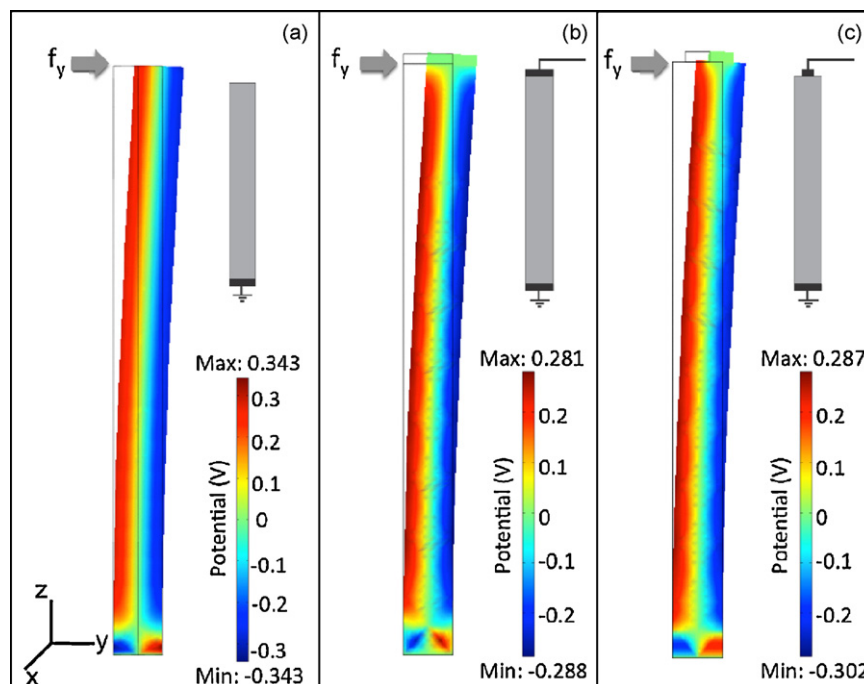
Fig. 2. Piezoelectric potential distribution (side view) in a top-bottom ZnO nanowire: TN-BT (a), TT-BT (b), TC-BT (c).
