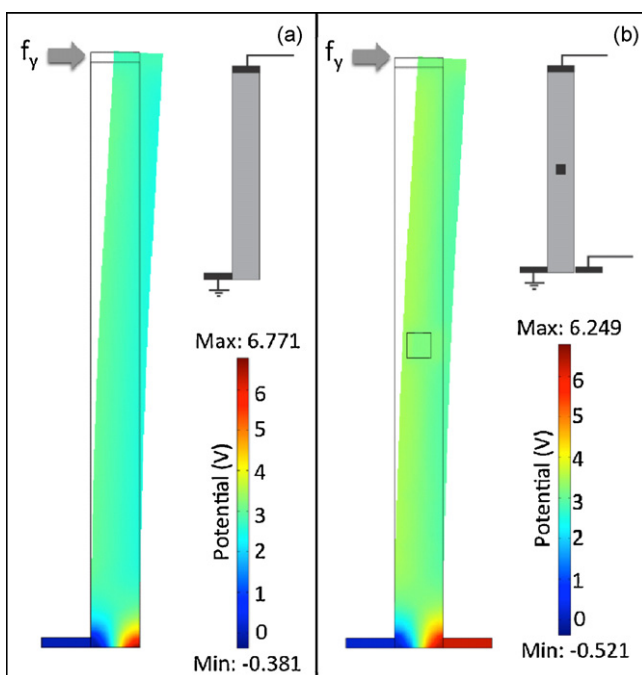
Fig. 4. Piezoelectric potential distribution (side view) in a bent bottom-bottom nanowire: BL (grounded)–TT (a); BL (grounded)–BC with TT and middle contact (b).
