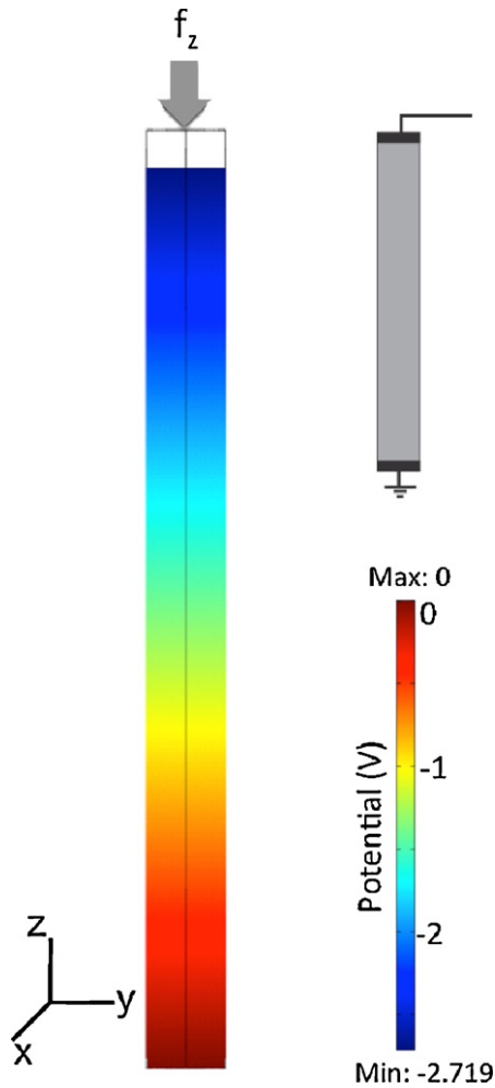
Fig. 5. Piezoelectric potential distribution (side view) in a compressed top-bottom nanowire (base totally short-circuited and base grounded).
