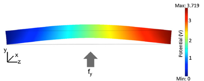
Fig. 6. Piezoelectric potential distribution (side view) of a laterally stretched piezoelectric nanowire.
