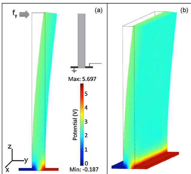
Fig. 8. Potential distribution of a bent bottom-bottom nanowall; (a) is a side view; (b) is a 3D view.
