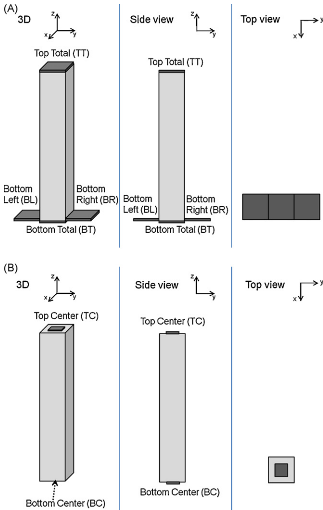
Fig. 1. (A) Definition of top-total (TT), bottom left (BL), bottom right (BR), and bottom total (BT) contacts. (B) Definition of bottom center (BC) and top-center (TC) contacts.
