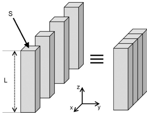
Fig. 7. Schematic representation of the equivalence between many nanowires connected in parallel and a single nanowall.
