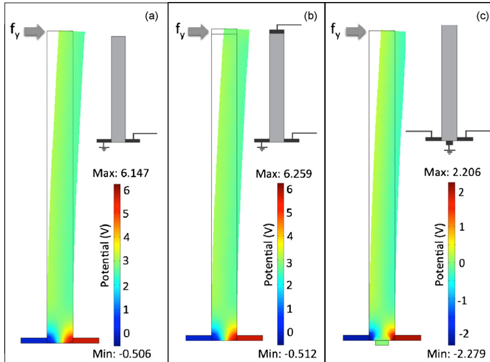
Fig. 3. Piezoelectric potential distribution (side view) in a bent bottom-bottom nanowire with various configurations: BL (grounded)–BR (a); BL (grounded)–BR with TT contact (b); BL–BR with TC (grounded) contact (c).
