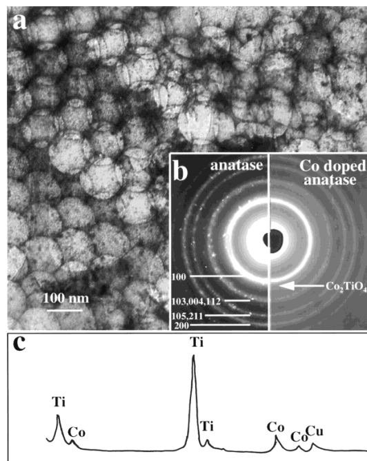
Fig. 4. a) A bright-field TEM image of the cobalt-doped anatase nanostructure, displaying the ordered structure. b) A comparison of the electron diffraction patterns between the host anatase (left-hand side) and the cobalt-doped anatase (right-hand side), where an extra ring (indicated by an arrowhead) is found in the pattern from the doped specimen, which may correspond to the \{220\} of \text{Co}_2\text{TiO}_4 . c) Energy dispersive X-ray spectrum shows the doping of cobalt into titania. The Cu signal comes from the Cu grid used in TEM.
