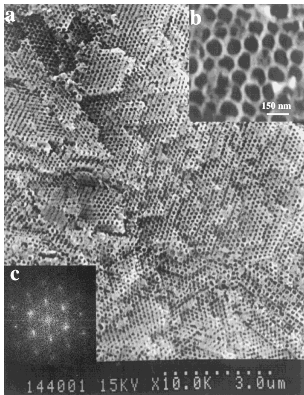
Fig. 1. a) A scanning electron microscopy image of the ordered porous nanostructure of anatase. b) An enlarged area showing the nanoporosity (diameter 90 \pm 10 nm) and the wall thickness of \approx 15 nm. c) A Fourier transform of the SEM image clearly shows the ordered pore structure with six-fold projected symmetry (the pixel used for Fourier transform was 512 \times 512 ).
