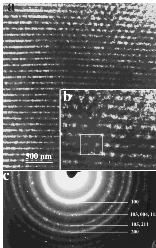
Fig. 2. a) A bright-field TEM image of the ordered pore structures. b) An enlarged area with the sketch of the projected [110] f.c.c. unit cell. c) A selected area electron diffraction pattern proves the anatase structure of titania. The rings are broadened due to the reduced size of the crystallites.
