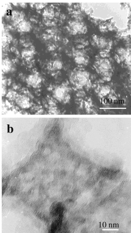
Fig. 3. a) A bright-field TEM image of the porous structure. b) A high resolution TEM image of anatase, showing the grain size of \approx 8 nm.
